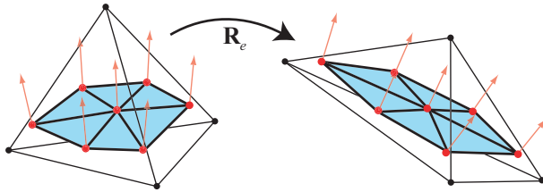
Figure 5: Vertices of the surface mesh are displaced according to the displacement field of the tetrahedron in which they lie. The rotation of the tetrahedron \mathbf{R}_e is used to rotate the normals.
