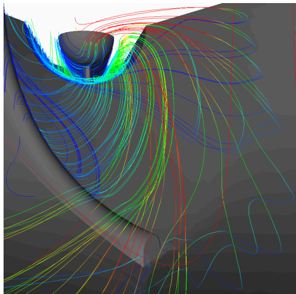
Figure 14: Close look at the first injector, field lines colored with distance to boundary. Some field lines follow the flow inside the injector while others connect to the boundary of the torpedo.
