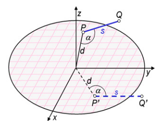
Figure 6: Filter lookup for the 3D line segment PQ by rotating the triangle OPQ onto the xy-plane.
