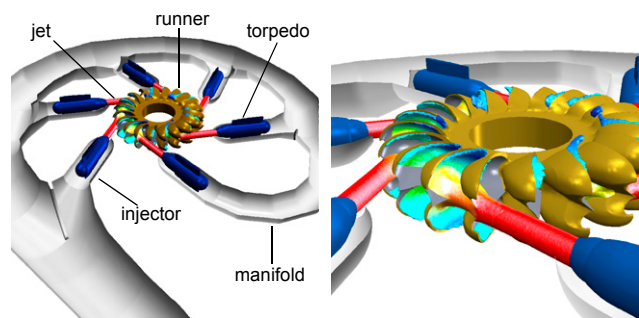
Figure 1: Pelton turbine: Manifold, injectors, torpedoes, jets and runner.
