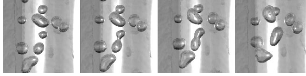
Figure 2: Small bubbles merge to larger bubbles due to surface tension forces.
