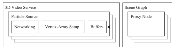
Fig. 3. 3D video service with video fragment sources and proxy object inside the scene graph. The buffers are used to pass data between the processes.
