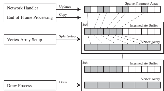
Fig. 6. Vertex array setup pipeline. The network process updates the fragment array and creates the intermediate copy in a job object for further processing. The vertex array setup process generates the vertex array data structure. Once the job object is ready, it is passed to the draw process.
