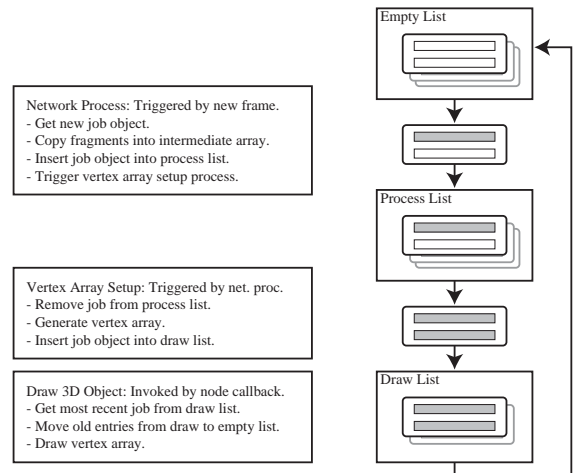
Fig. 7. Job processing in the vertex pipeline. Job objects are stored in lists for processing. The setup process is triggered by the previous stage in the pipeline using a semaphore.
