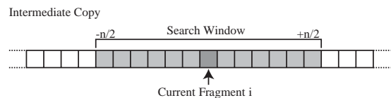
Fig. 9. Nearest-neighbor window search method. For each fragment i , the distance between the fragment and each of the previous n/2 and next n/2 is calculated. The smallest distance is used as the splat radius if it is below a threshold.
