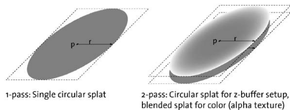
Fig. 5. Splat rendering: single pass and two-pass rendering modes. Circular splats are rendered with a quad primitive and an alpha texture as stencil. The same alpha texture is used for blending. p denotes the fragment position, r the size of the splat.
