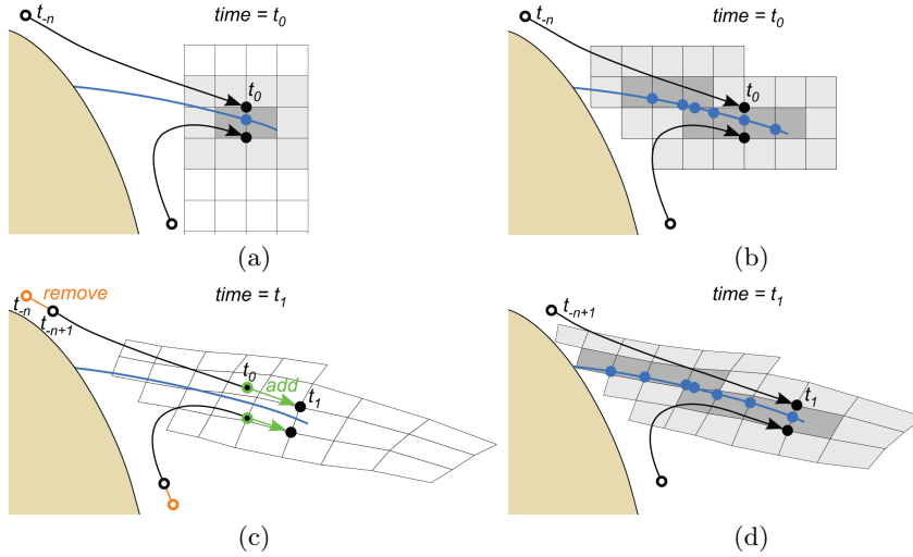
Fig. 2. Grid advection for flow separation. (a) Initial sampling grid. Ridge cells (dark gray) and their neighboring cells (light gray). Cell edge intersected by negative-time FTLE ridge (blue point). Neighborhood range is 1 for illustration purposes. (b) After grid adaptation. (c) After one step of grid advection. (d) After grid adaptation of advected grid.
