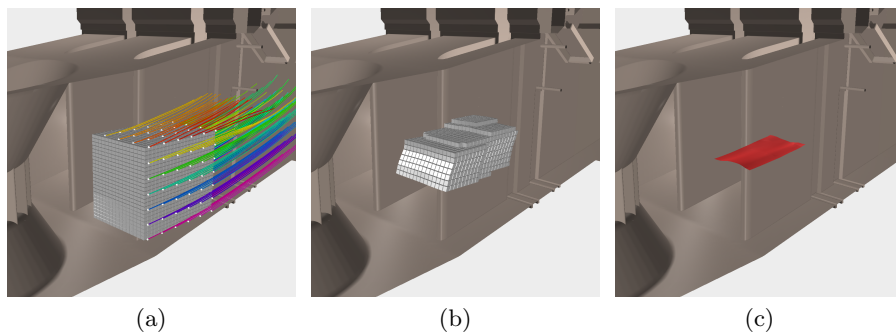
Fig. 5. Intake of a water turbine. (a) Uniform grid with some of the upstream trajectories (colored) used for FTLE computation, and their seeds (white spheres). (b) Sampling grid adapted to ridge region and advected. (c) Resulting FTLE ridge.
