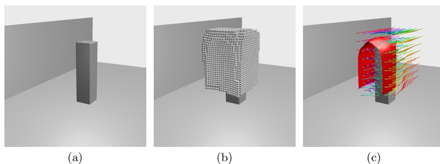
Fig. 4. Flow around a cuboid. (a) Geometry. (b) Sampling grid adapted to ridge region and advected. (c) Resulting FTLE ridge with some upstream trajectories (colored) from uniform grid, and their seeds (white spheres).
