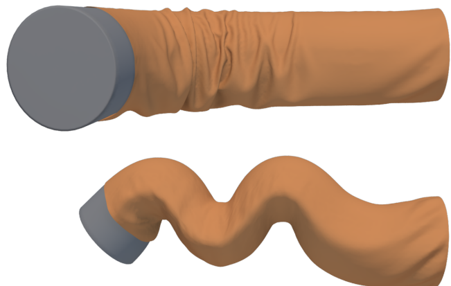
Figure 8: When simulating this cloth with a PSDB featuring only motions in the horizontal plane, our method reproduces plausible wrinkling when bending the left end of the tube to the front (top). When moving to a pose very far from the training data, our solver produces deformations very close to the skinned basis (bottom).
