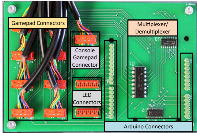
Figure 9: Custom-designed multiplexing hardware for eight NES gamepads.
