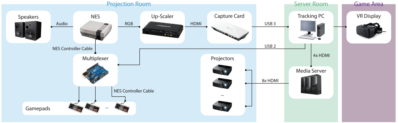
Figure 2: System architecture overview. The NES output video signal is first captured and sent for analysis. The tracking PC processes the video stream, tracks the background, and creates a wide, panoramic image. This image is either incorporated into a VR environment or sent to a 360 degree projection system. The projection system receives the video streams, processes, and outputs them to the projectors. For the projection configuration, the division between the projection hall and server room is indicated by blue and green backgrounds, respectively.
