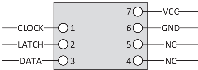
Figure 7: NES gamepad cable pinout.
